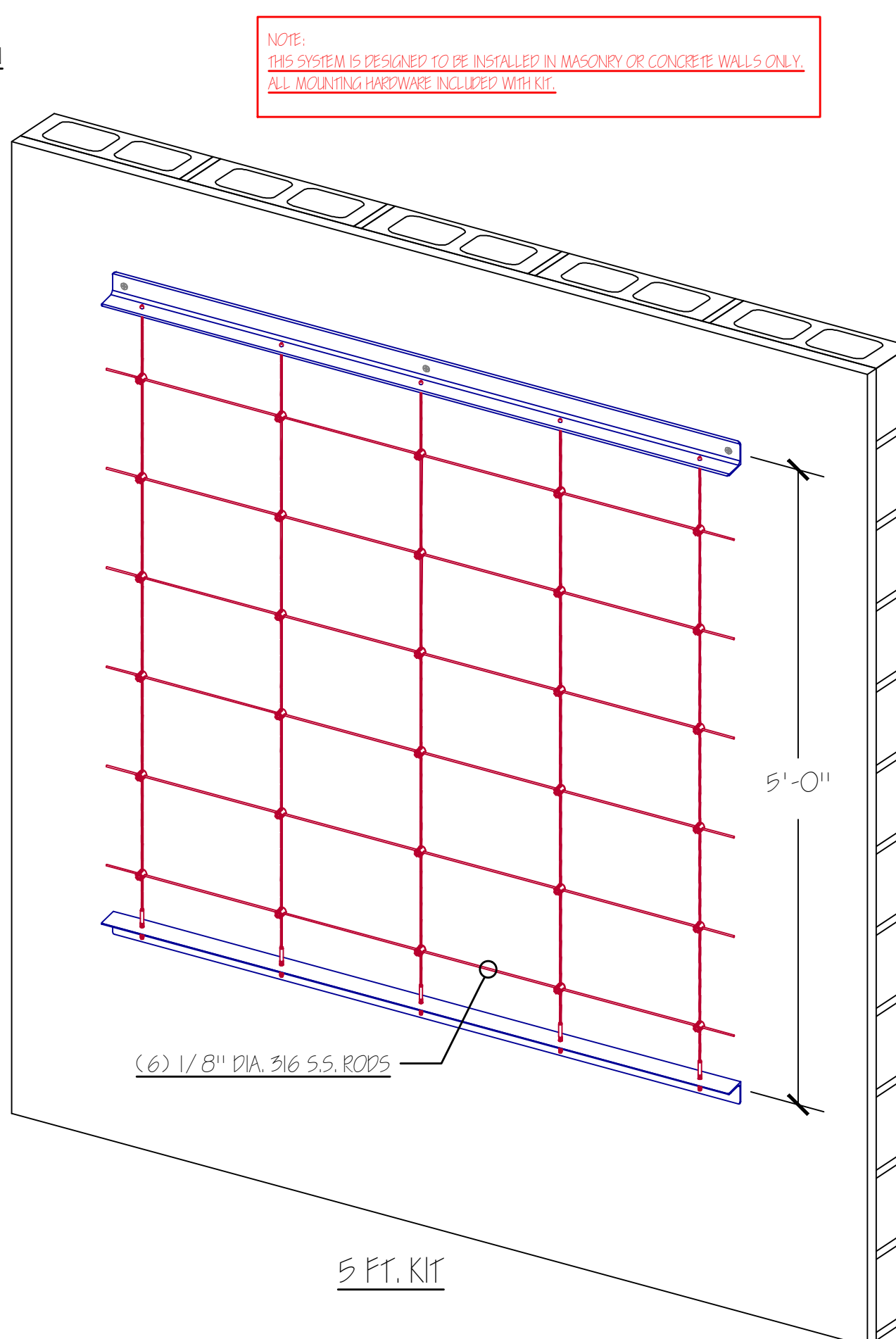
WALL GARDEN TRELLIS - ISOMETRIC VIEWS N.T.S.
