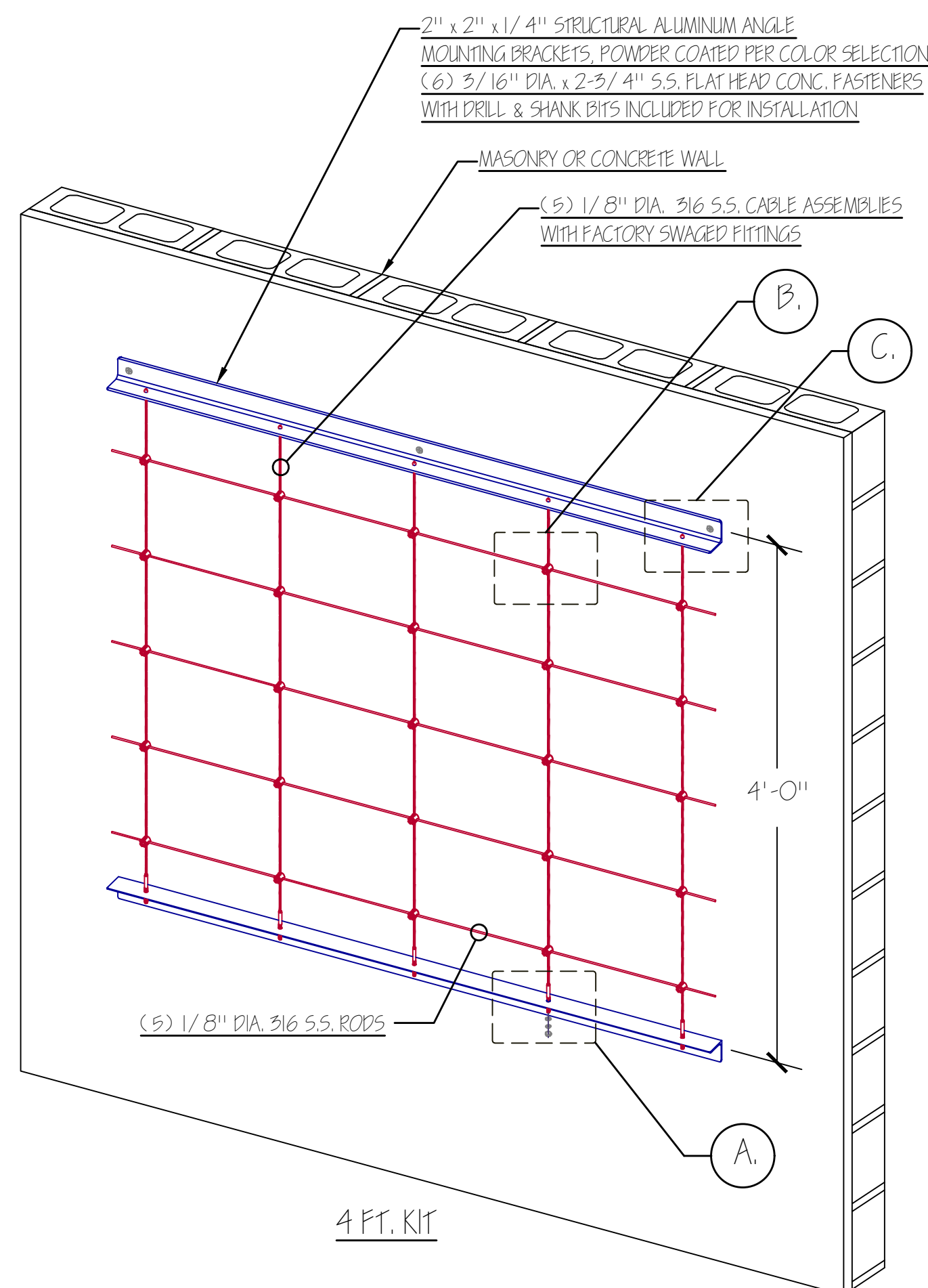
WALL GARDEN TRELLIS - ISOMETRIC VIEWS N.T.S.
