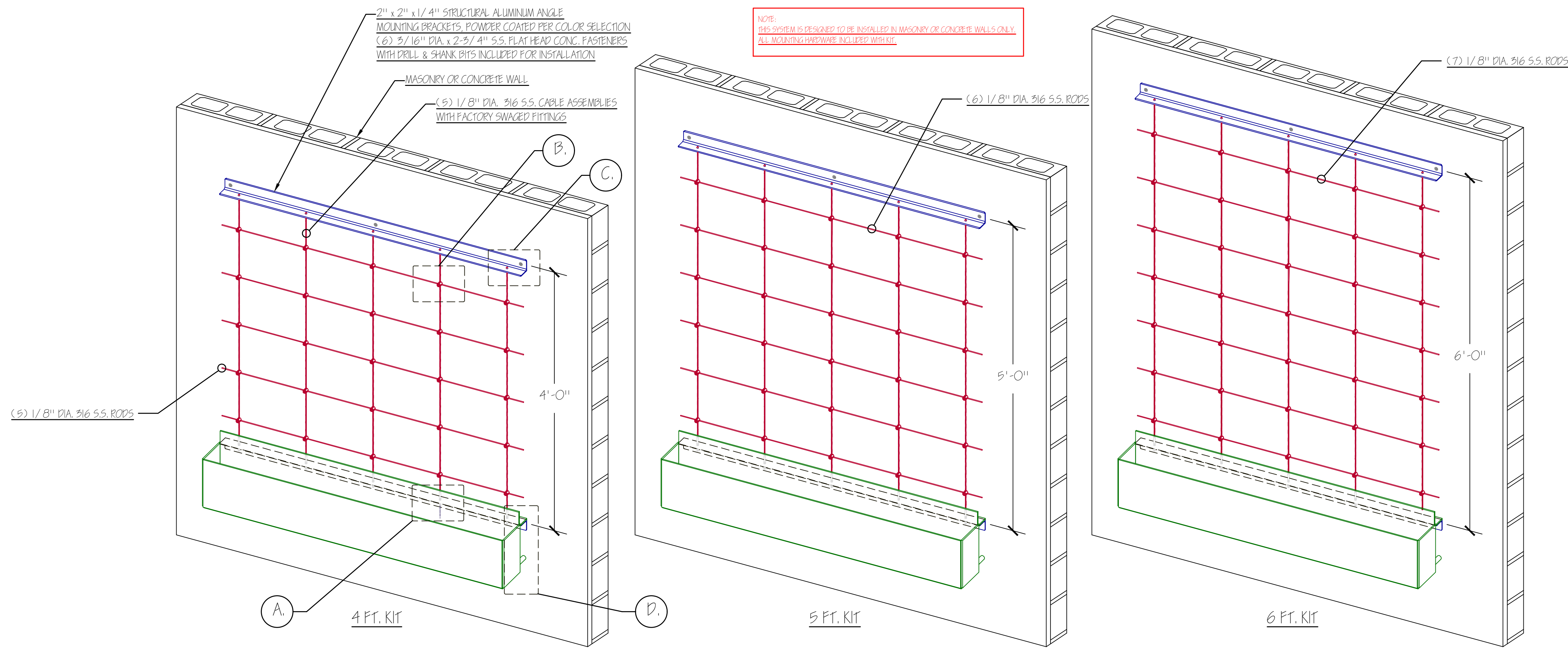
WALL GARDEN TRELLIS WITH PLANTER BOX - ISOMETRIC VIEWS N.T.S.
